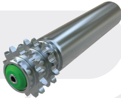
1306 series – Double sprocket rollers
